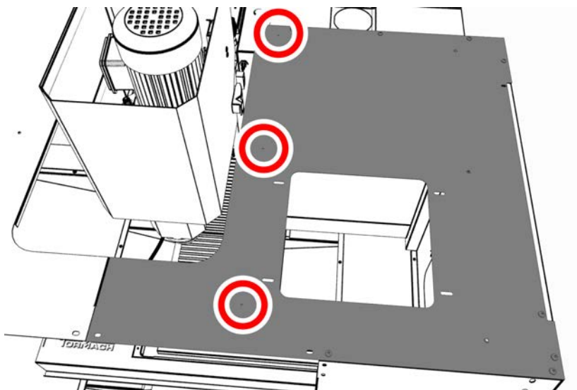
Figure 14: Location to attach three cable tie anchors.
