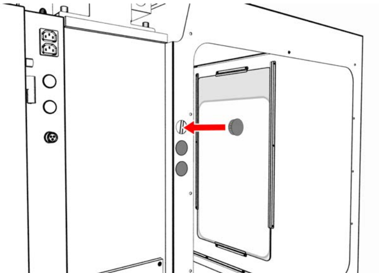
Figure 34: Round hole plugs pushed into the left rear panel.
