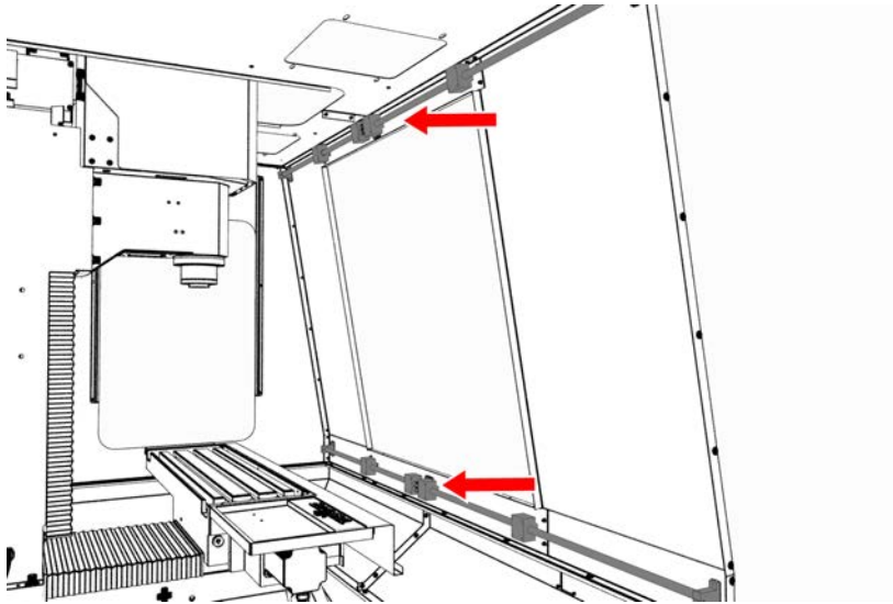
Figure 22: Four linear assemblies attached to the enclosure.
