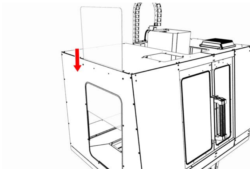
Figure 32: Window sliding into the window opening.
