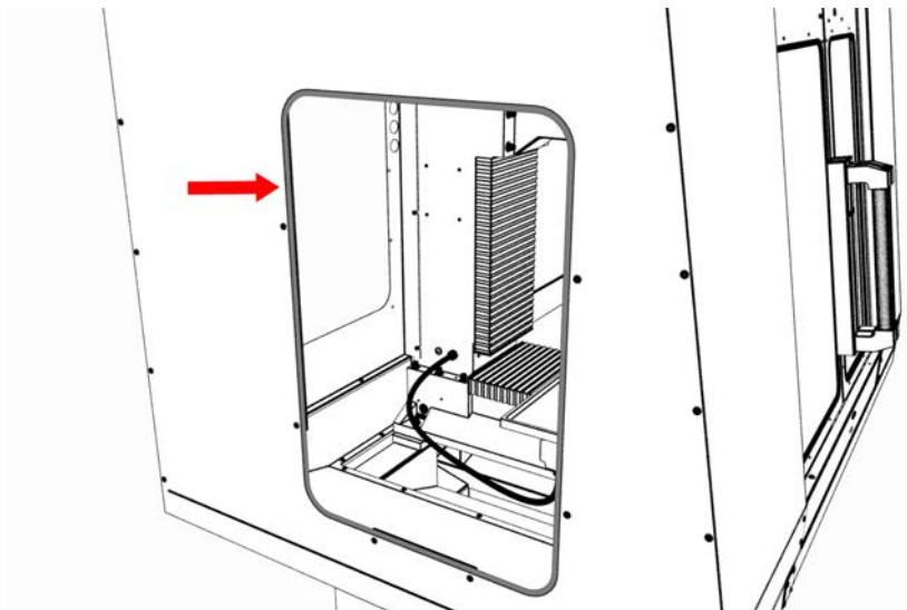
Figure 31: Rubber trim pushed onto the window opening.
