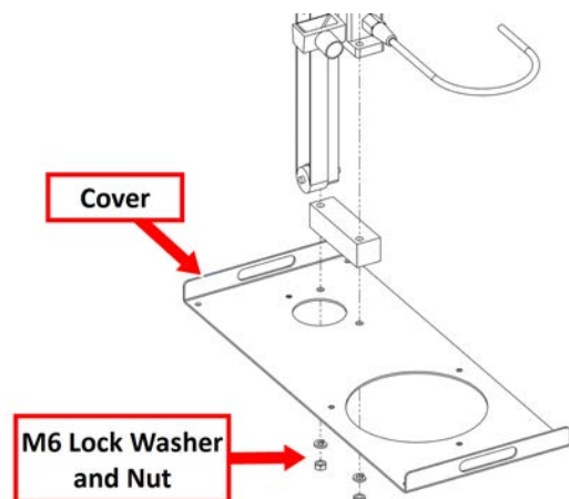
Figure 3: Securing the skimmer to the skimmer plate.
