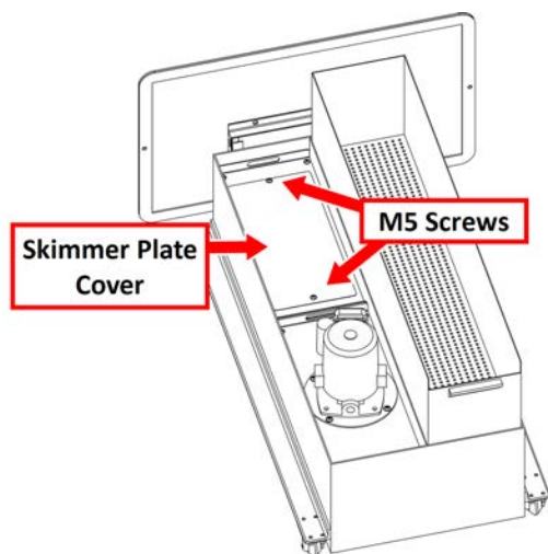
Figure 1: Skimmer plate cover on the skimmer plate.
