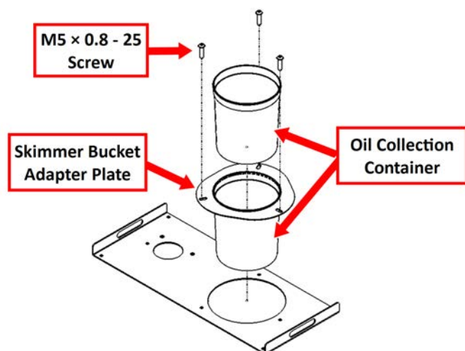
Figure 4: Securing the oil collection container to the skimmer plate.
