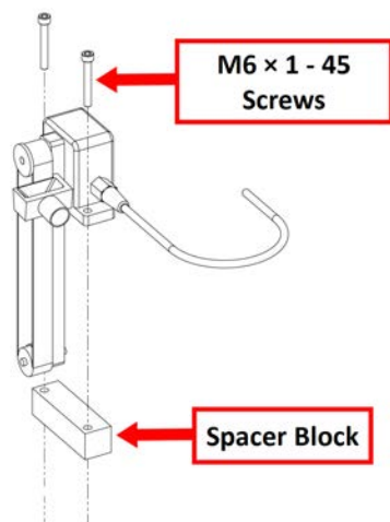
Figure 2: Securing the skimmer to the mounting block.
